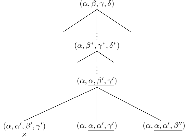
FIGURE 7. We are once again simulating a two-dimensional walk between the underlined nodes. The fact that (\alpha, \alpha', \beta', \gamma') is terminal follows from Lemma 4.17.
