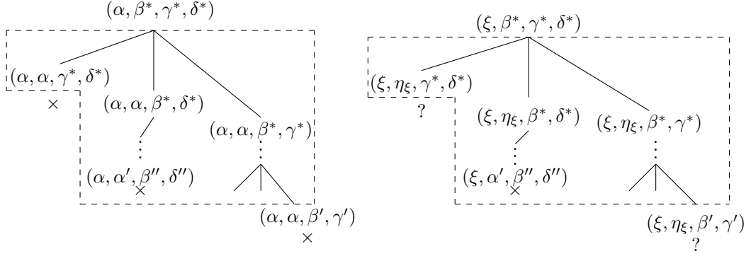
FIGURE 9. The bad case. By Lemma 4.21, the parts of S_3(\alpha, \beta^*, \gamma^*, \delta^*) and S_3(\xi, \beta^*, \gamma^*, \delta^*) that lie within the dashed lines are the same.
