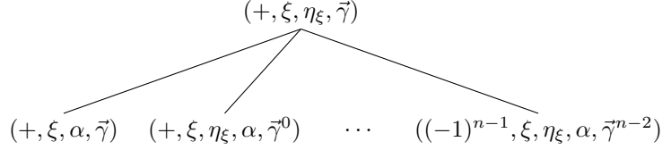
FIGURE 18. The \xi -image of the bad case when \alpha \in \text{nacc}(C_{\bar{\gamma}}) .
