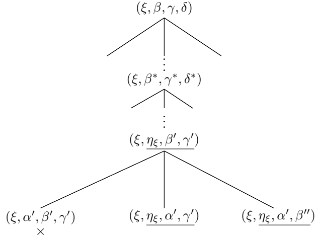
FIGURE 8. Node (\xi, \alpha', \beta', \gamma') is terminal by Lemma 4.17.
