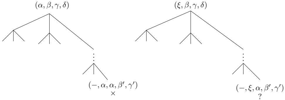
FIGURE 10. The good case. We have assumed for definiteness that the starting node is (\alpha, \beta, \gamma, \delta) . Here, the left and the right trees are the same, by Lemma 4.10.
