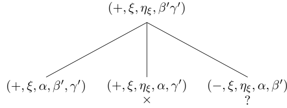
FIGURE 14. If \xi > \bar{\alpha} , then \eta_\xi \notin C_{\beta'\gamma'} and \min(C_{\beta'\gamma'} \setminus \eta_\xi) = \alpha .
